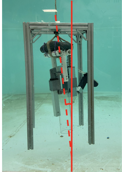
Fig. 17. Image displays testing of the version two of the sampler in the test tank. Red annotations point out the angle of descent of the sampler and its deviation from the vertical.
