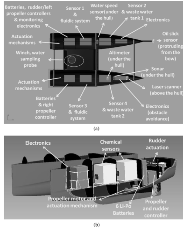
Fig. 3. Layout and mechanism of Hydronet ASV provided in publication. [11]
