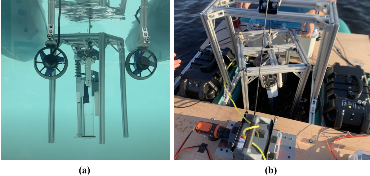
Fig. 15 (a) Successful test of winch system in Sea Grant tank. (b) River testing of the winch system, where currents rotated the sampler which caused the frame to catch on the plywood.
