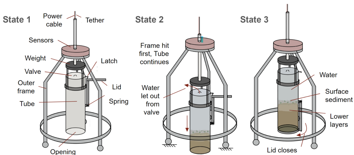
Fig. 10. Sketch of the first iteration of the sediment core sampling system. The whole assembly slowly lowers to the ground together (State 1) until they reach the seafloor. The frame contacts the ground first and provides stability, while the tube continues to fall. The tube drops to the ground with enough force to dig into the sediment (State 2), and when it lifts up, the lid swings down to enclose the sample (State 3). The cysts are located in the top layers of the surface sediment.
