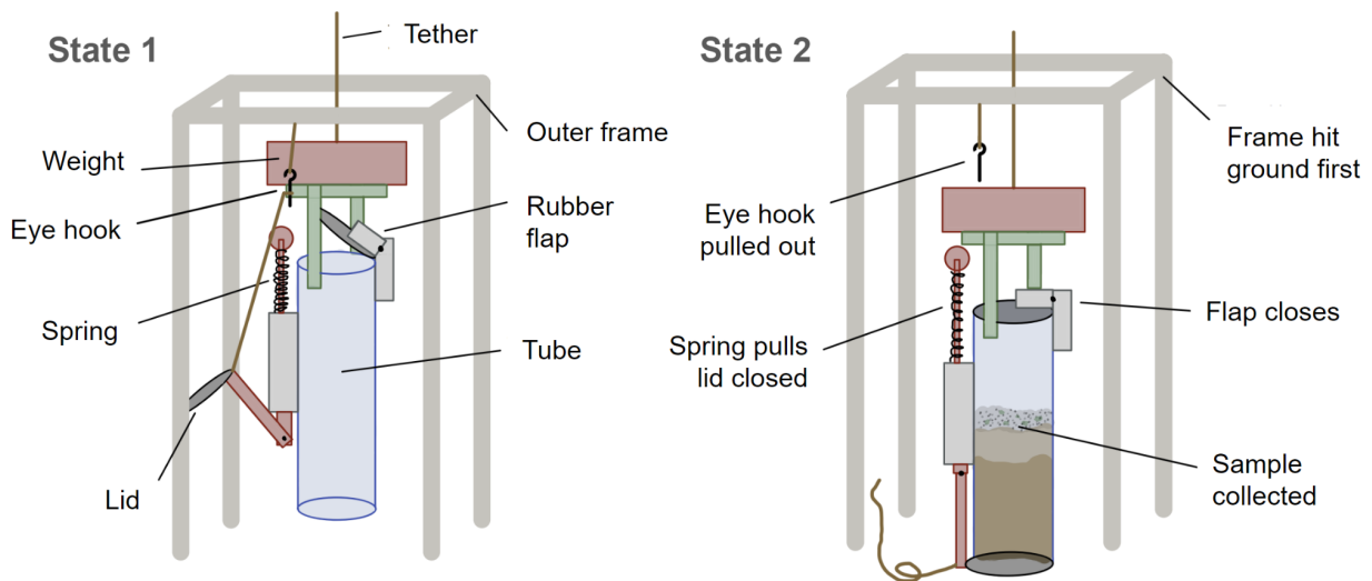
Fig. 11. Sketch of the second iteration of the sediment sampler design. The spring swings the lid down to seal the bottom of the tube and continues to pull upward, securing it in place. State 1 shows the preloaded position of the sampler, in which it gets deployed and travels to the seafloor. In State 2, the tube descends farther than the outer frame, pulling out the eye hook and closing the lid.
