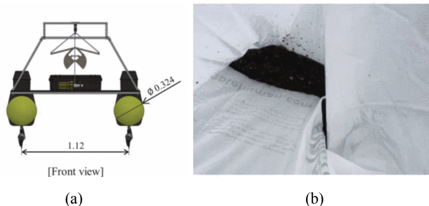
Fig. 2. (a) Model of unmanned surface vehicle shown with a Van Veen grabber for sediment collection. (b) Photograph of a collected sediment sample [10].
