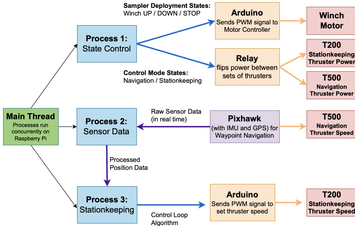
Fig. 13. Control Block Diagram depicting the flow of signal between the computational logic performed in processes run on the Raspberry Pi and Arduino microcontrollers, Pixhawk, and relays that interface directly with the motors.
