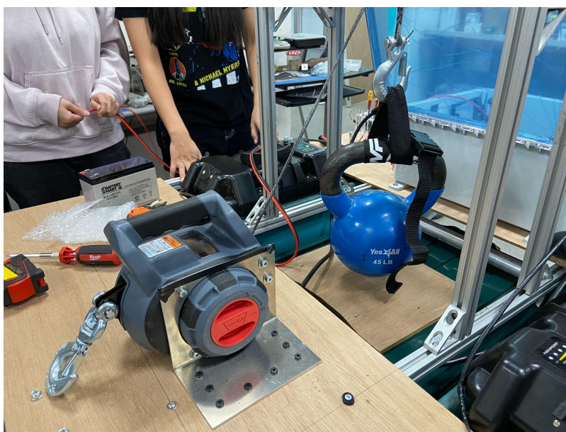
Fig. 14. The winch system doing a test deployment with a 45 lb weight
