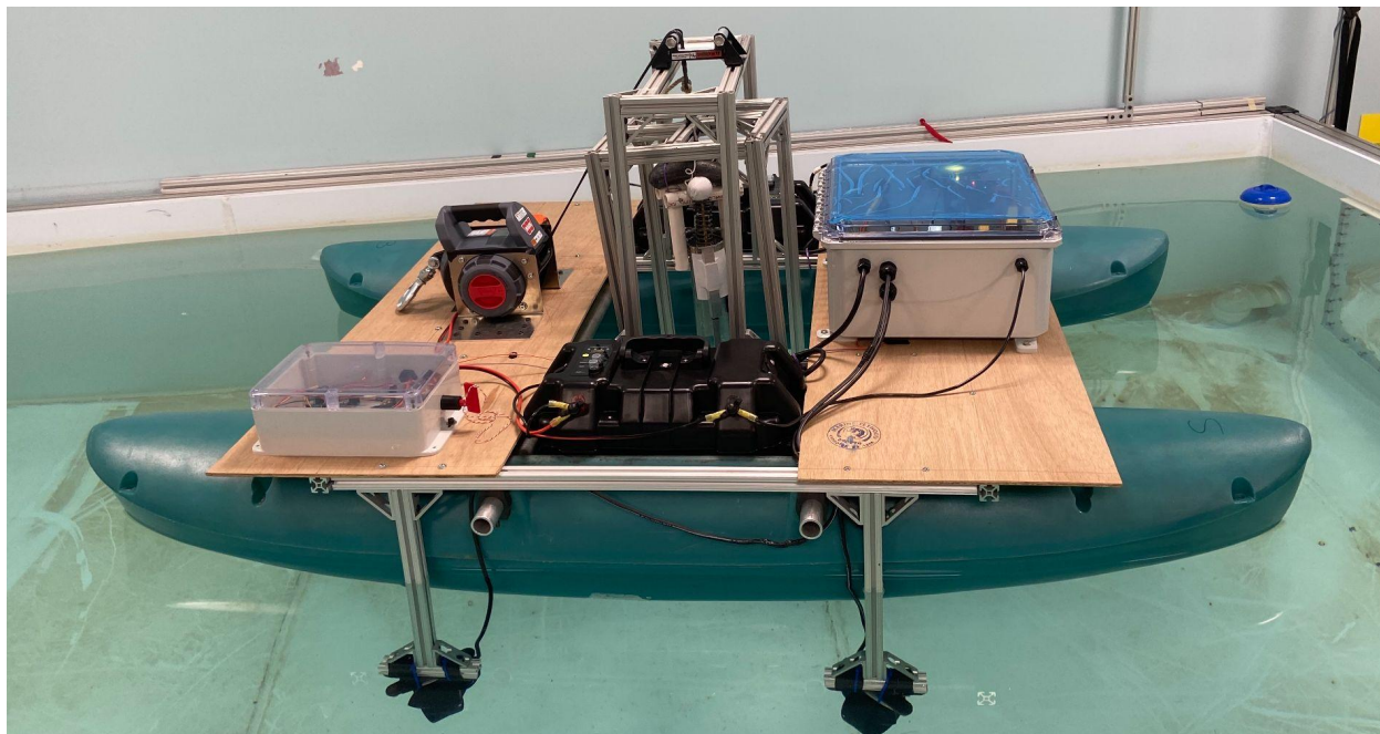
Fig. 18. The fully integrated system during indoor tank testing
