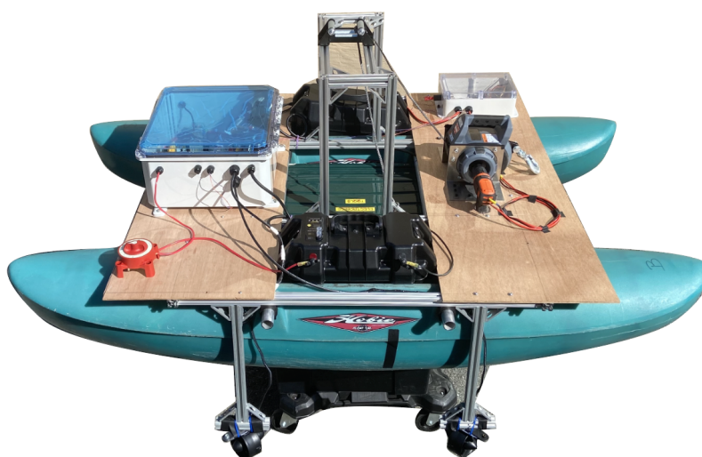
Fig. 9. Completed platform, including electronics boxes, batteries, winch, and sampling frame.
